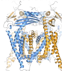
TRPML1 by cryo-EM
